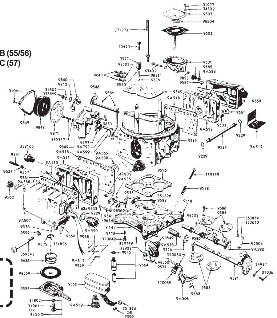
1957 CARBURETOR
