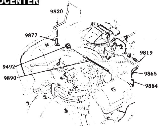
56/57 CHOKE
